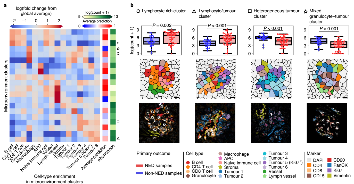
Fig. 4 | Clustering of SPACE-GM embeddings identifies disease-relevant microenvironments. a , A total of 20 clusters are identified by fitting a K -means clustering ( K = 20 ) on microenvironment embeddings. The heatmap on the left shows different cell-type enrichment patterns in microenvironment clusters. The column in the middle shows the average prediction values for the primary outcome task from each cluster of microenvironments; note that the colour scale is different from the enrichment matrix. The column on the right shows the abundance of each cluster of microenvironments in the UPMC-HNC dataset. The black shapes on the right indicate the specific cell clusters shown in b . Circle, a lymphocyte-rich cluster; star, a tumour cell and myeloid cell (granulocytes and macrophages) cluster characterized by mixed spatial distributions; diamond, a
